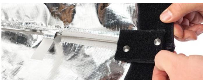
5.) Attach the Velcro® strips to the end of the SNAPBAG®. Make sure the SNAPBAG® is on full tension by utilizing the Velcro® strips before installing the diffuser.
