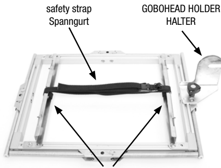
adapter brackets / Adapter-Klauen
